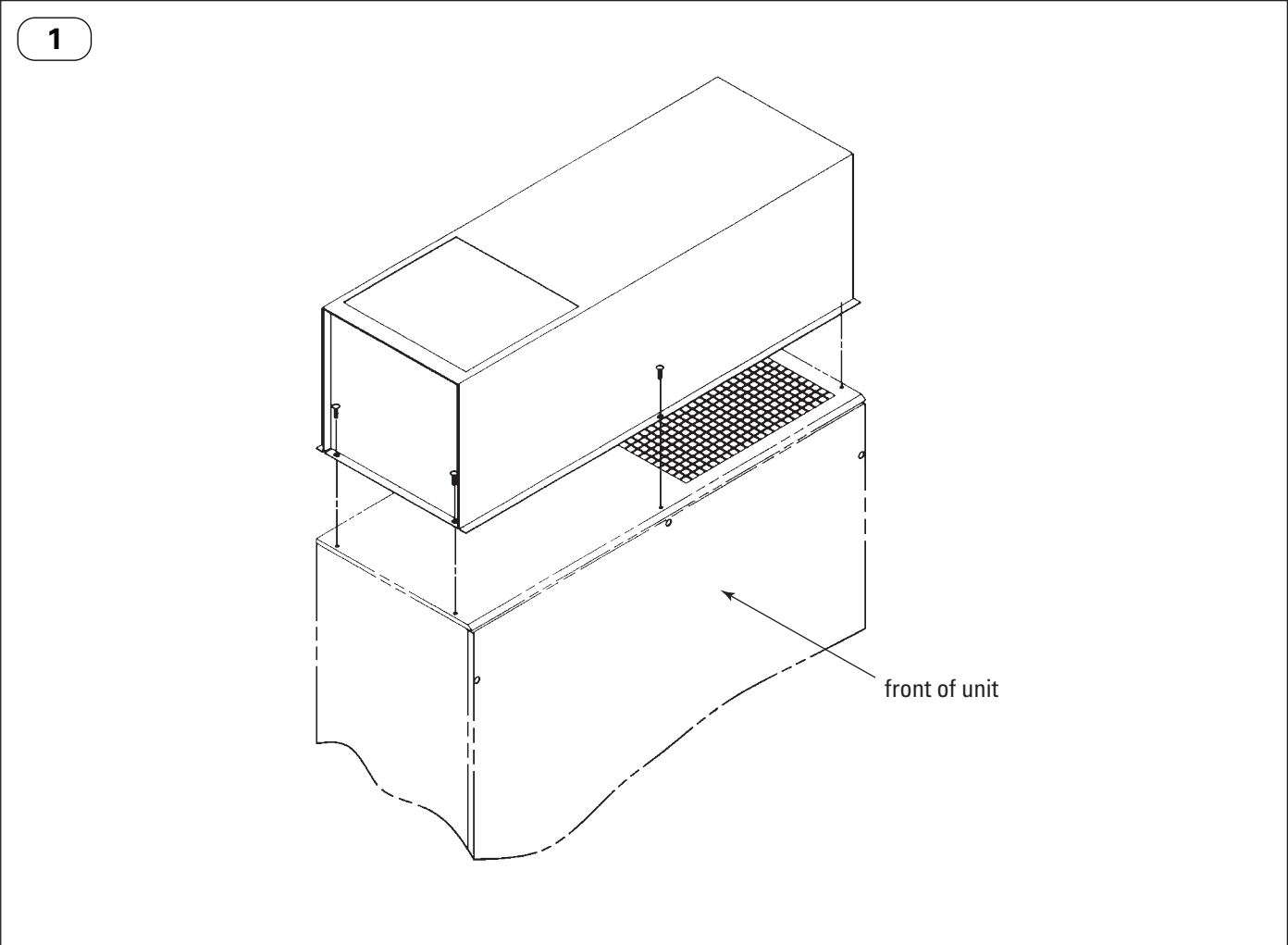
Silencer Assembly
