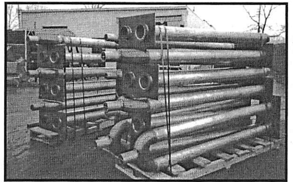
Fabricated T-330 Radiant Tube Assemblies
