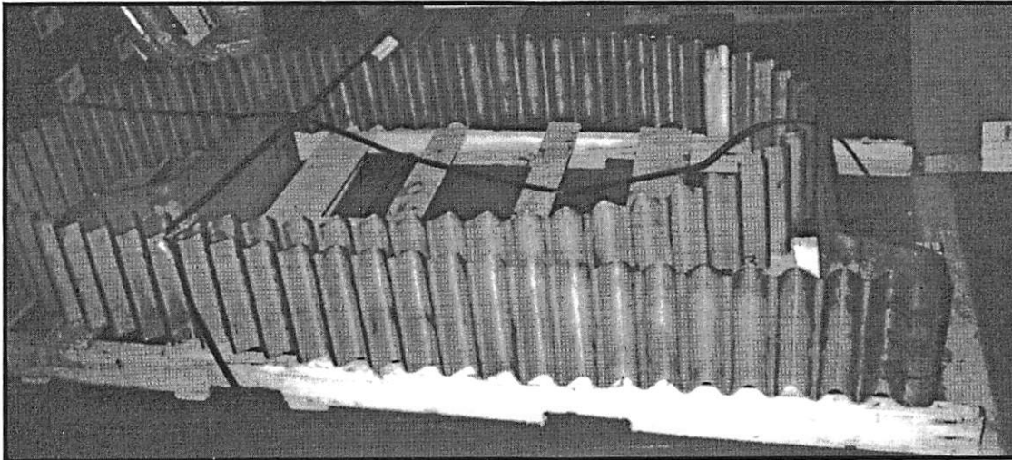
Corrugated Inconel® 600 Heating Element for Pit Carburizing Furnace
