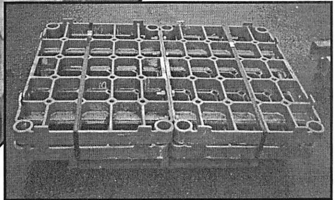
Cast HU Alloy 36"x48" Furnace Trays
