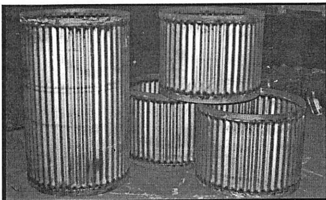
Fabricated T-330 Alloy Corrugated Furnace Shrouds
