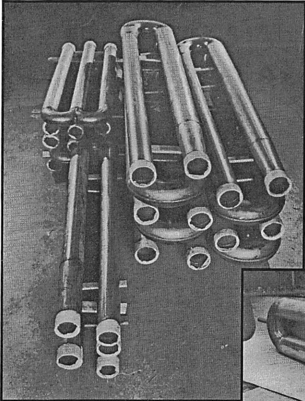
Fabricated T-330 Alloy Straight, "U" and "W" Style Radiant Tube Assemblies
