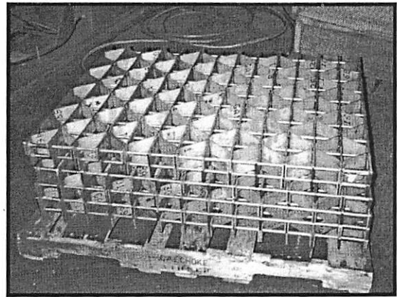
Special Vacuum Tray Fabricated of MA 956® Load Bars and Inconel® 600 Serps and Tie Rods
