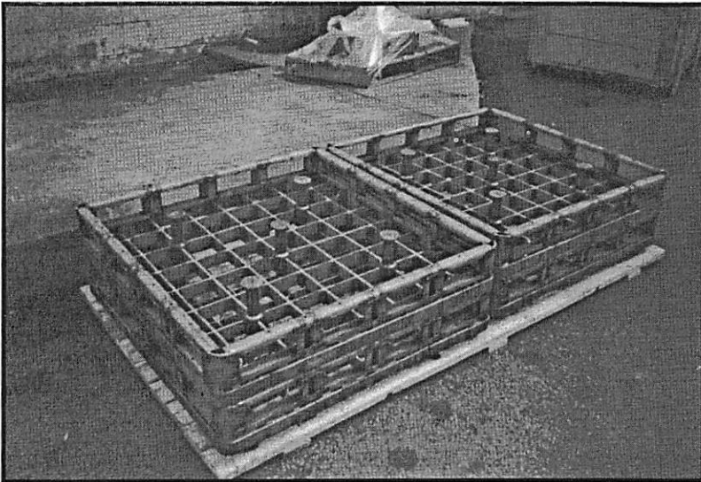
Fabricated Incoloy 800® Fixtures for Gears and Bearings
