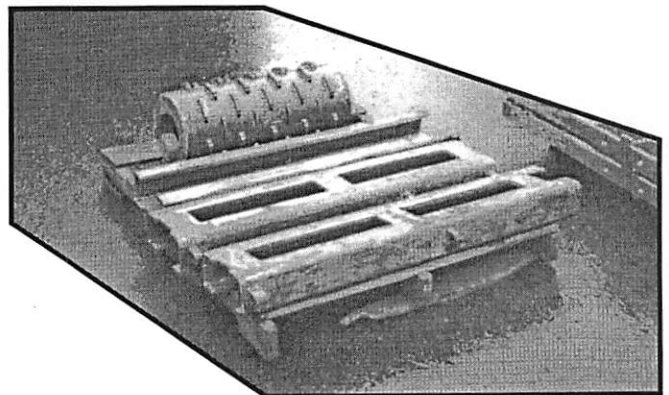
Cast HT Alloy Chain Guides and Cast HH Alloy Furnace Drum
