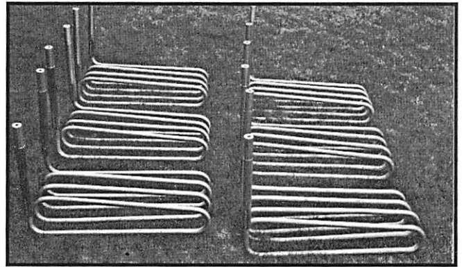
Fabricated T-330 Alloy Pipe Heating Elements for Allcase® Furnace
