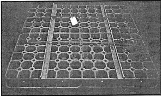
Cast HX Alloy 39"x42" Reversible Furnace Trays
