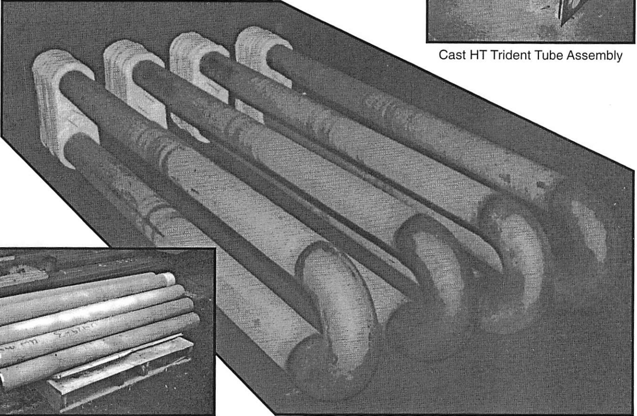
Centrifugally Cast HN Alloy Tubes
