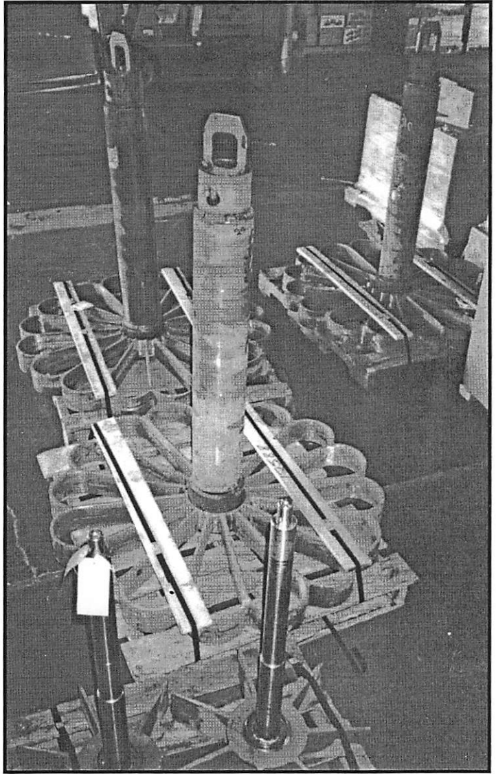
Cast HT Alloy Center Post Lifting Fixtures Cast & Fabricated HT/330 Alloy Fan Assemblies
