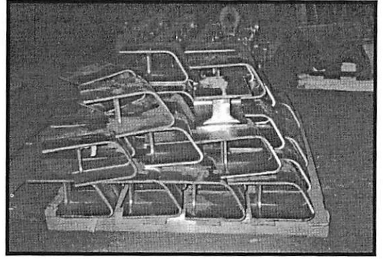
Cast HH Alloy Diffusers for Bell Anneal Furnace
