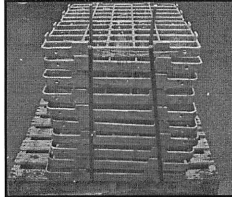
Cast HU Alloy 24"x36" Furnace Trays
